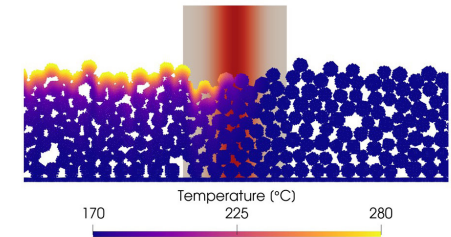
Figure 1: QR code for the process window app (left); underlying PBF-LB/P simulation for polyamide 12 (right).
