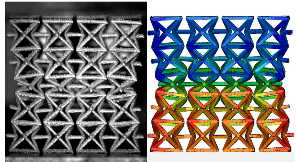
Drop weight test: 17,6 kg, 5 m/s, dynamic equilibrium.
