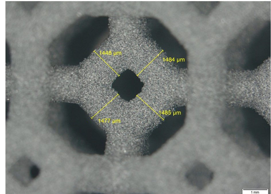
Detailed picture of a printed gas burner structure
